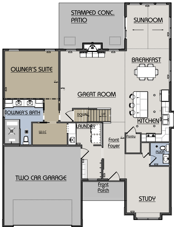
Main Floor
